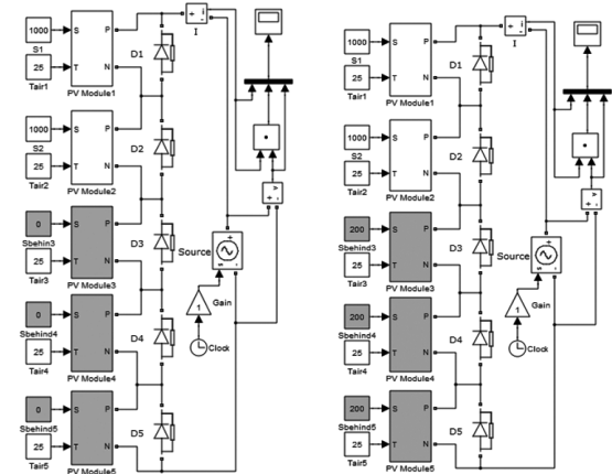
(a) $S_{chech\alpha n} = 0W/m^2$; $T_{air} = 25^\circ C$
