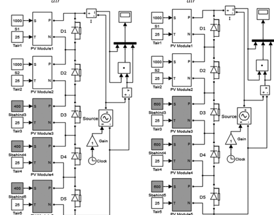
(c) $S_{chech\alpha n} = 400W/m^2$; $T_{air} = 25^\circ C$
